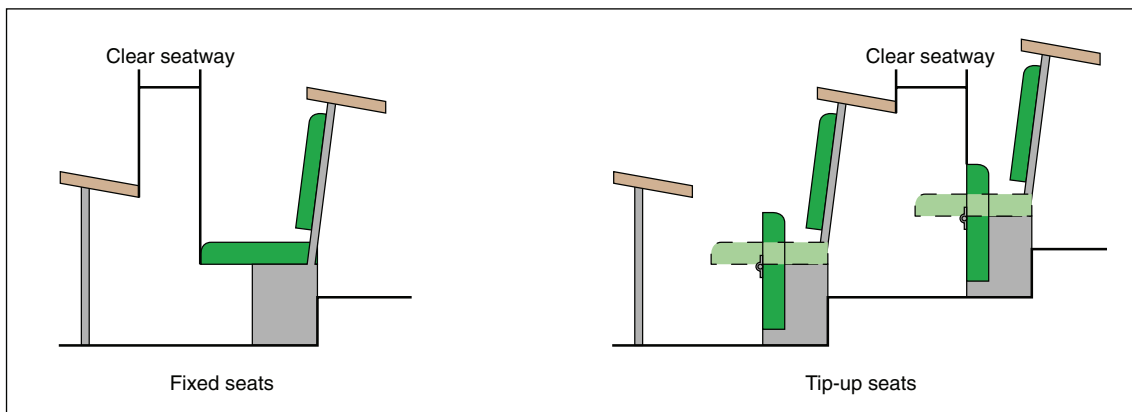
Figure 22: Clear space between seating
