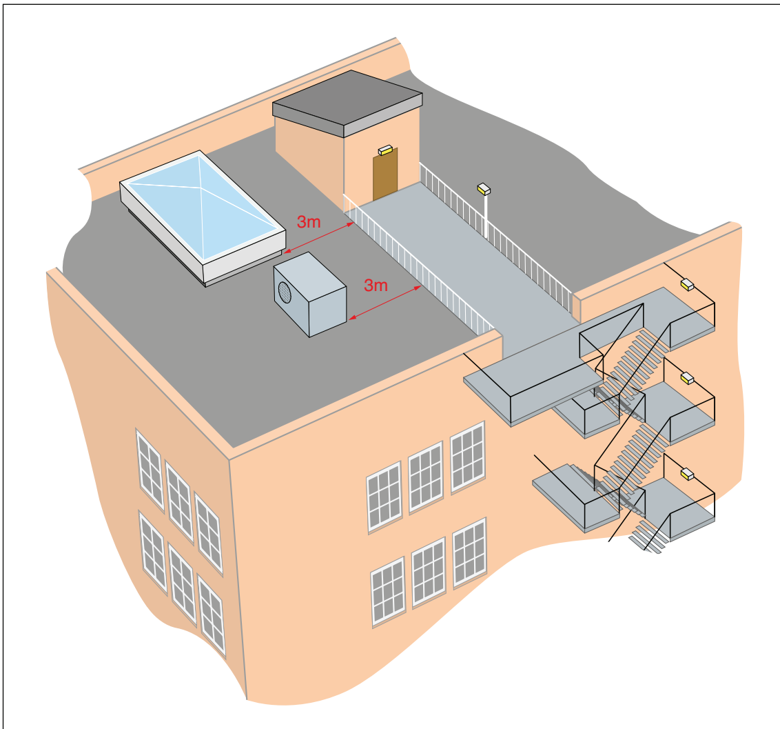
Figure 43: An escape route across a roof
