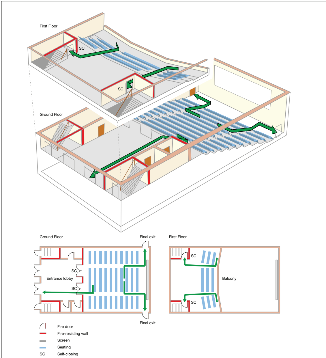
Figure 50: Two-storey (ground and balcony)
