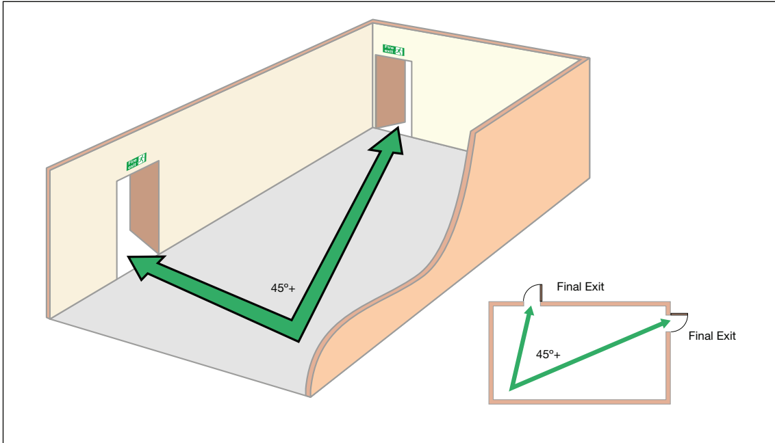
Figure 26: Alternative exits
