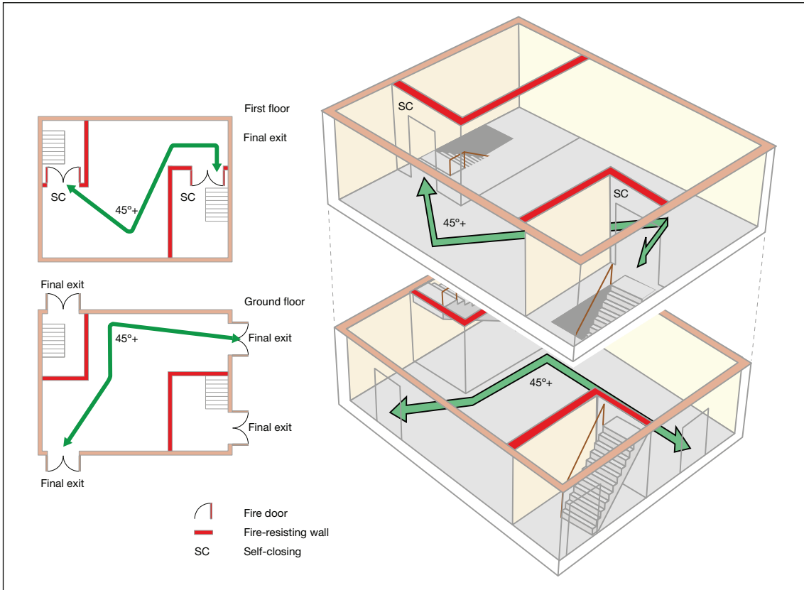
Figure 49: Two-storey (ground and first floor)
