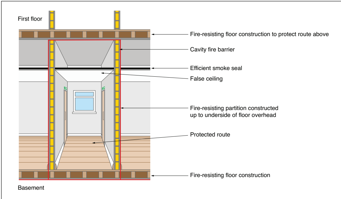
Figure 67: Fire-resisting construction
