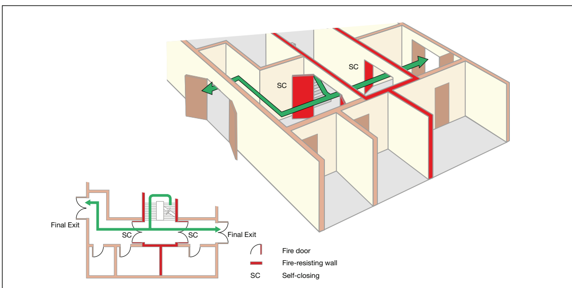
Figure 37: Example of two escape routes from a stairway to final exits
