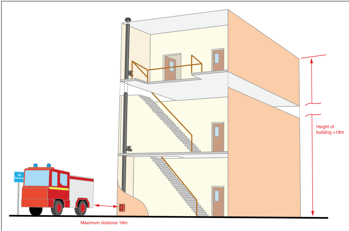
Figure 21: Rising main
