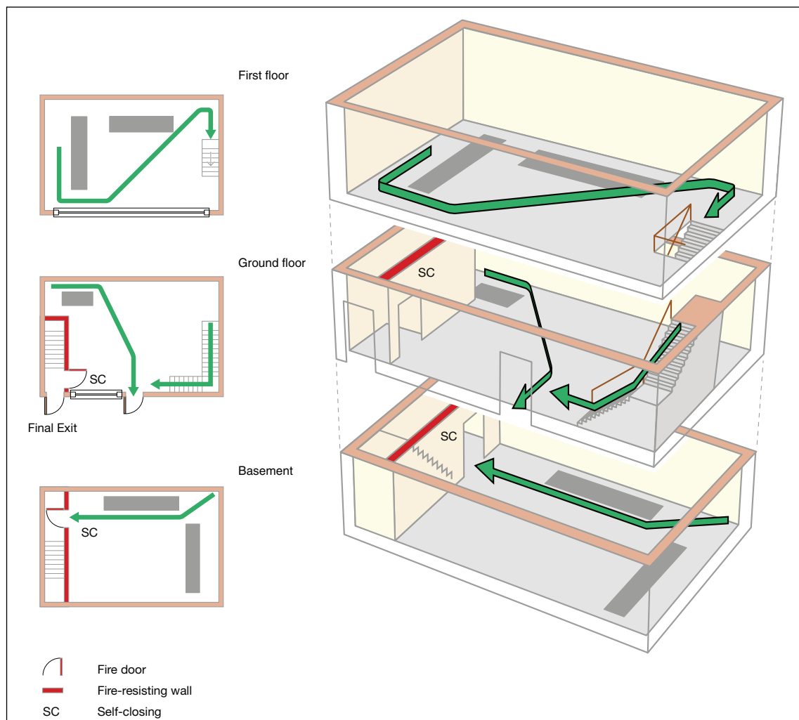
Figure 55: Three-storey (small basement, ground and first floor)
