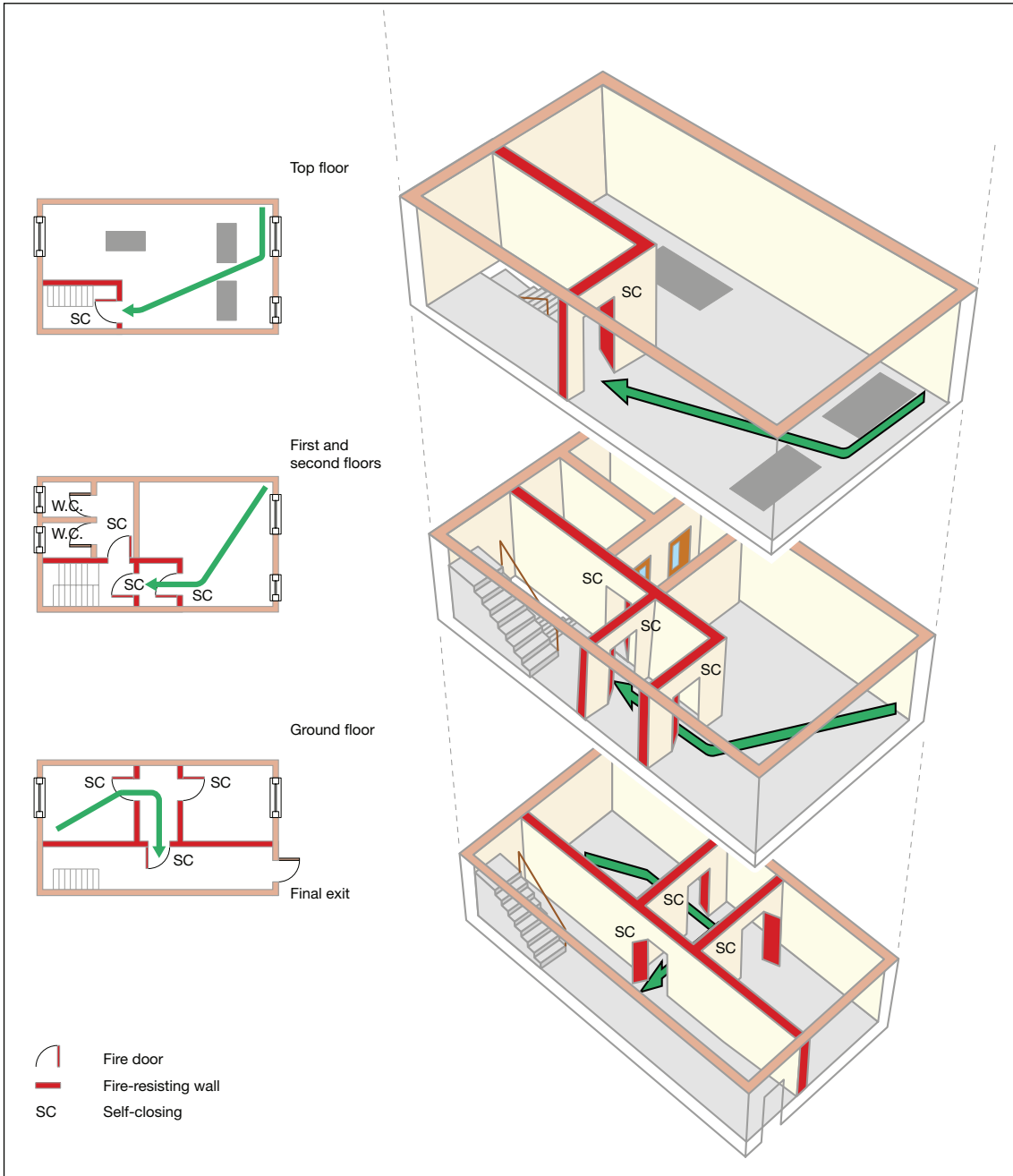
Figure 57: Four-storey, ground and up to three upper floors – protected by lobbies/corridors
