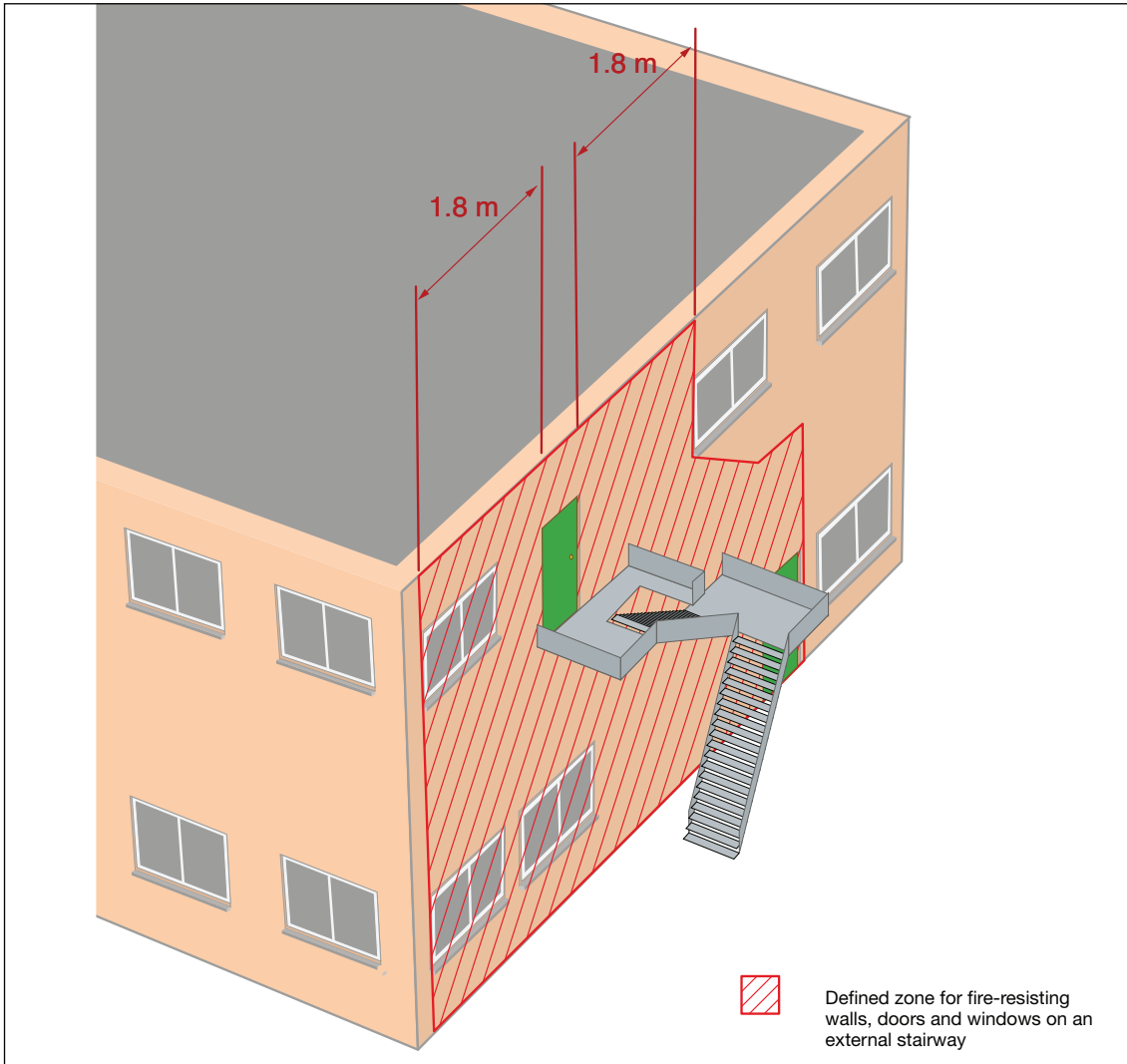
Figure 42: Protection to an external stairway
