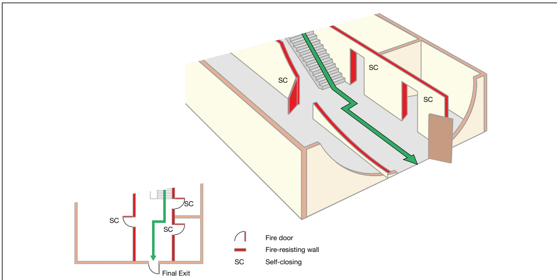
Figure 36: Example of a protected route from a stairway to a final exit
