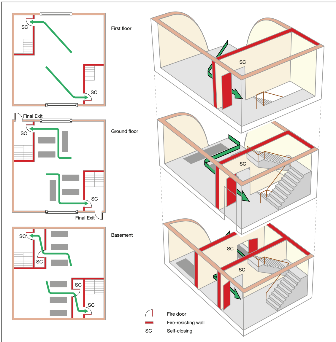
Figure 51: Three storey (basement, ground and first floor)
