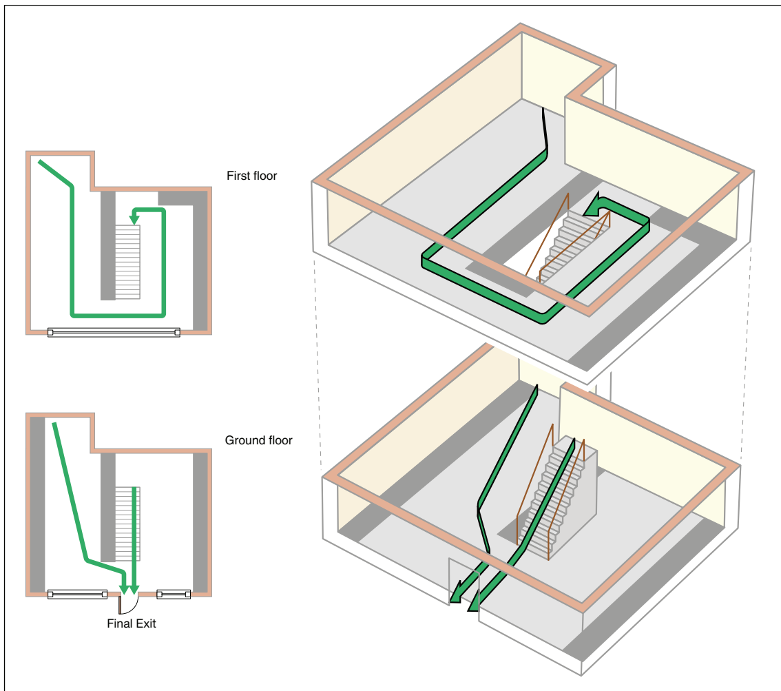
Figure 53: Two-storey (ground and first floor)
