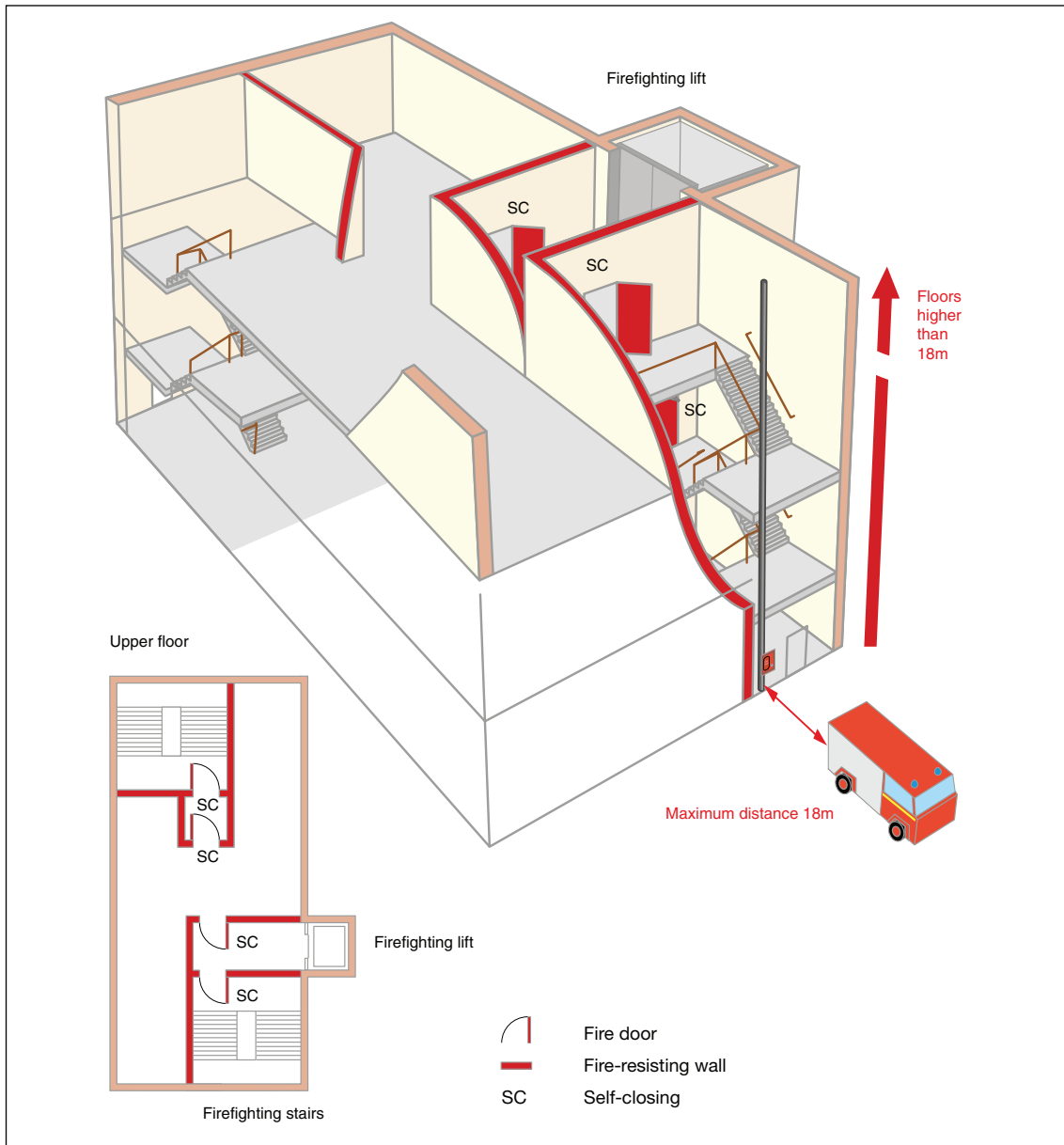
Figure 52: Tall building with a firefighting shaft
