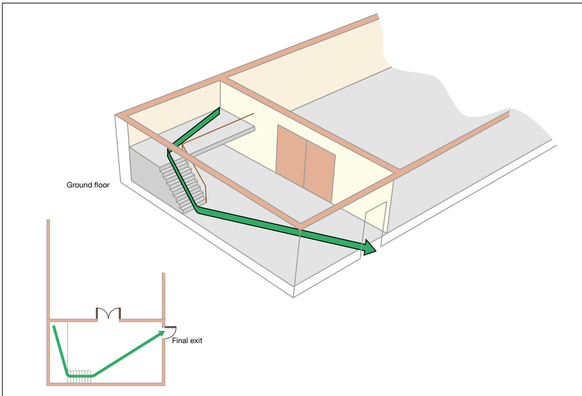
Figure 47: Single storey with a single exit (including a mezzanine)
