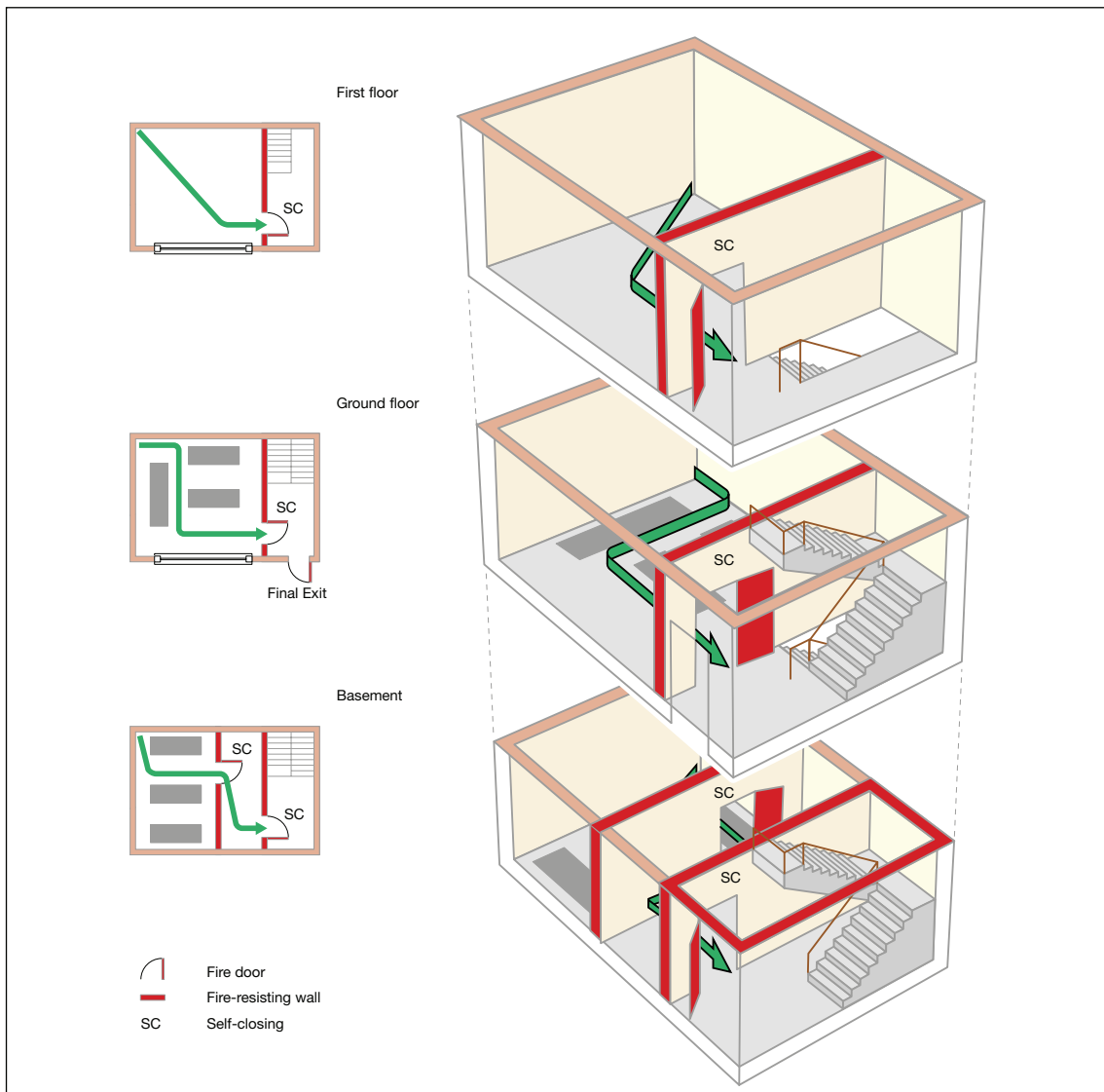
Figure 56: Three-storey (basement, ground and first floor)
