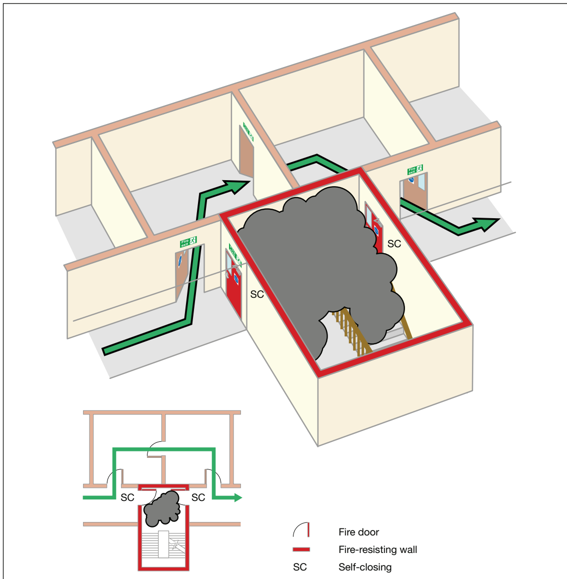
Figure 39: A stairway bypass route
