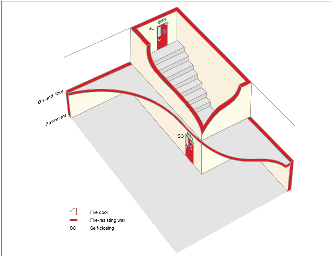
Figure 33: Basement protection
