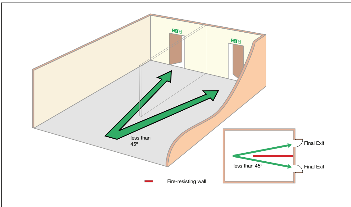
Figure 27: Alternative exits separated by fire-resisting construction
