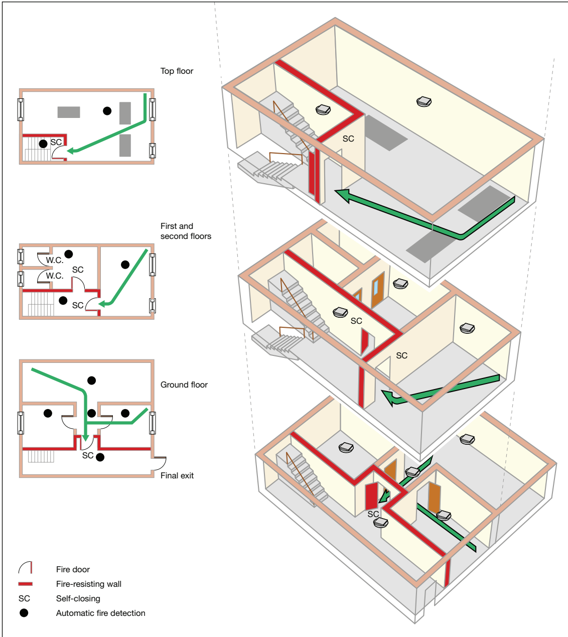
Figure 58: Four-storey, ground and up to three upper floors – protected with automatic fire detection
