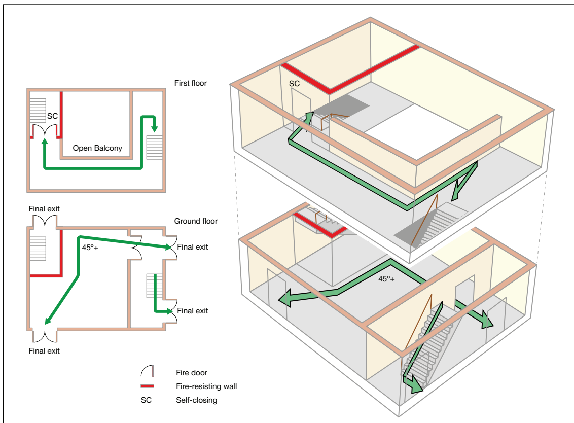
Figure 48: Two-storey (one protected and one open stairway)
