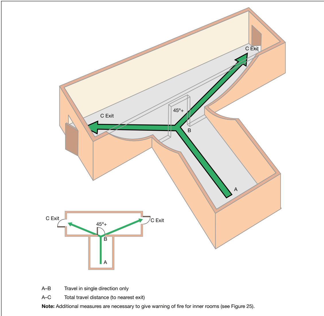
Figure 29: Measuring travel distance from initial dead end (inner room)
