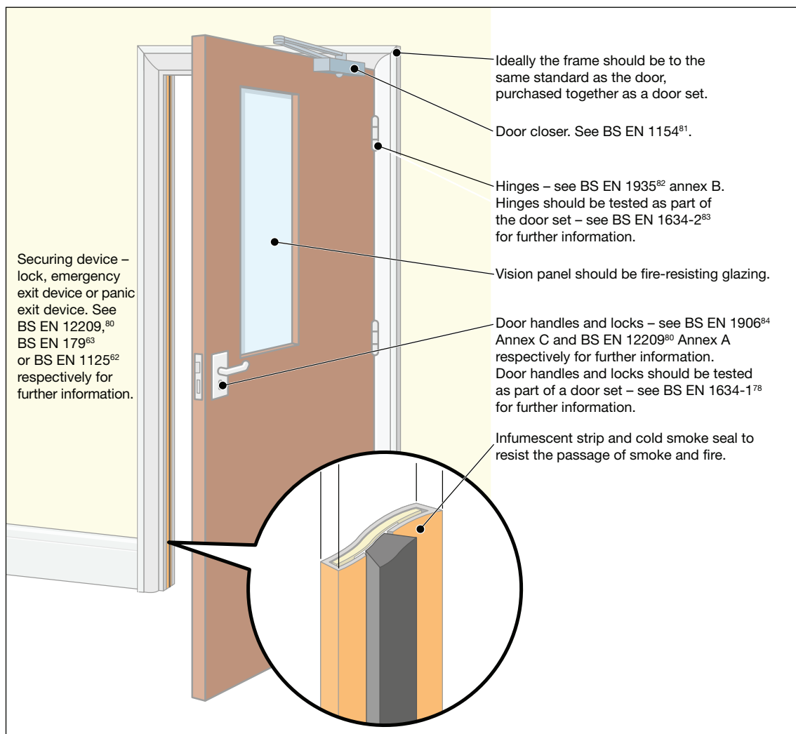
Figure 68: A fire-resisting and smoke stopping door
