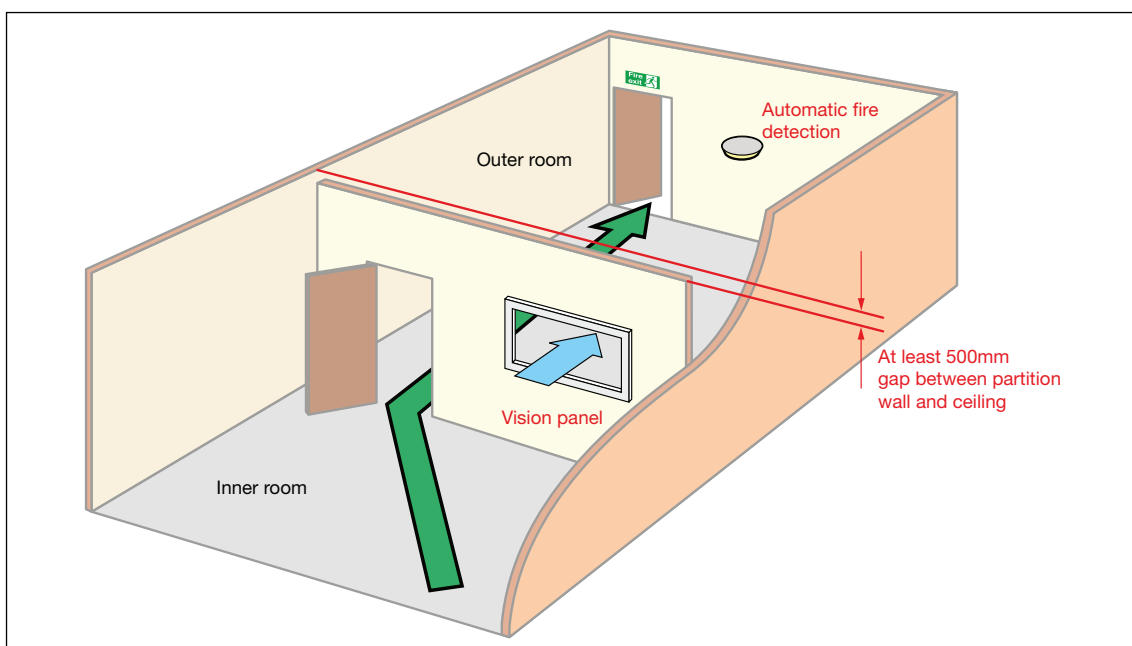
Figure 25: Inner rooms
