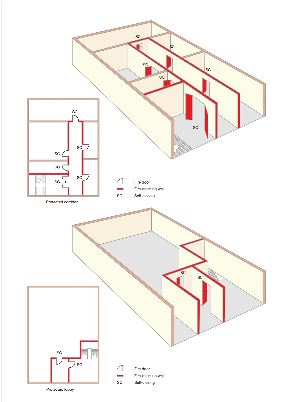
Figure 35: Examples of a stairway with protected lobby/corridor approach
