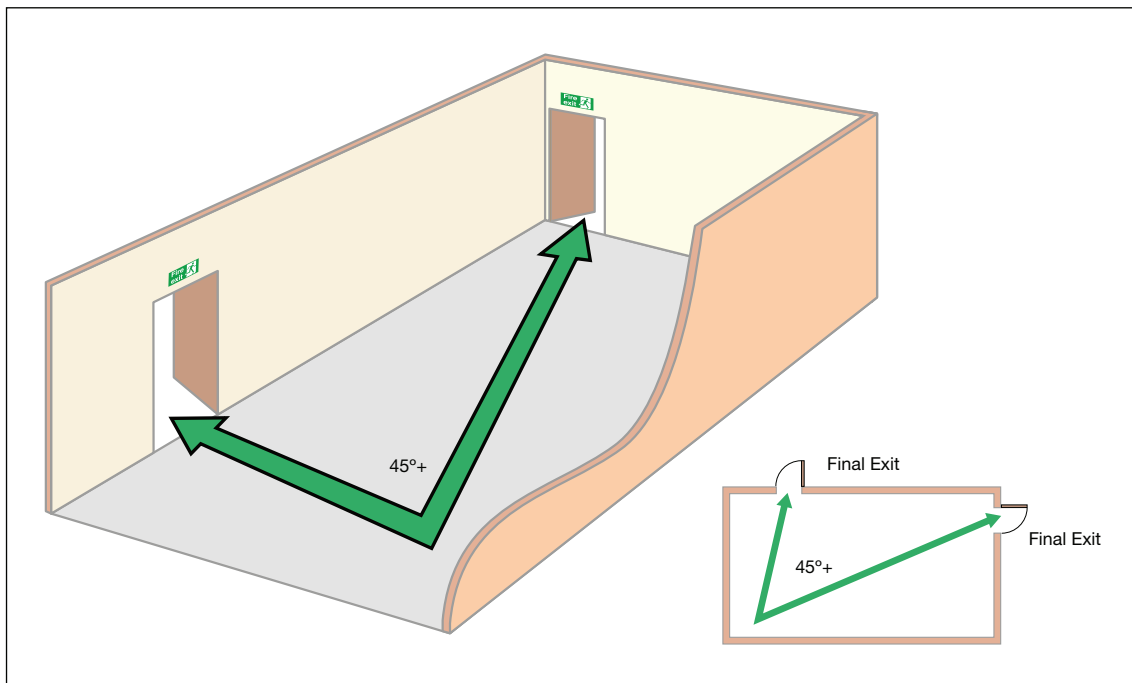
Figure 44: Ground floor with more than one exit
